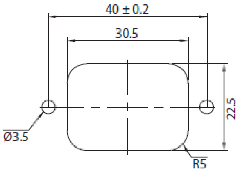
FOR REAR MOUNTING USE PANEL CUTOUT
