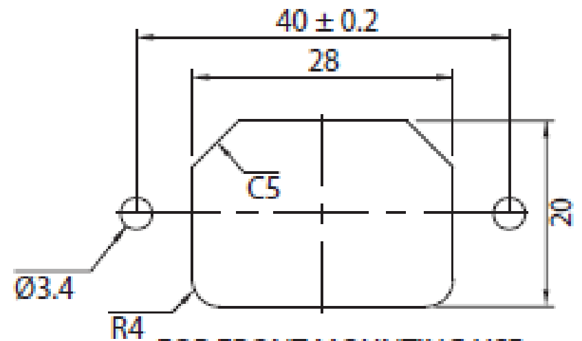
FOR FRONT MOUNTING USE PANEL CUTOUT
